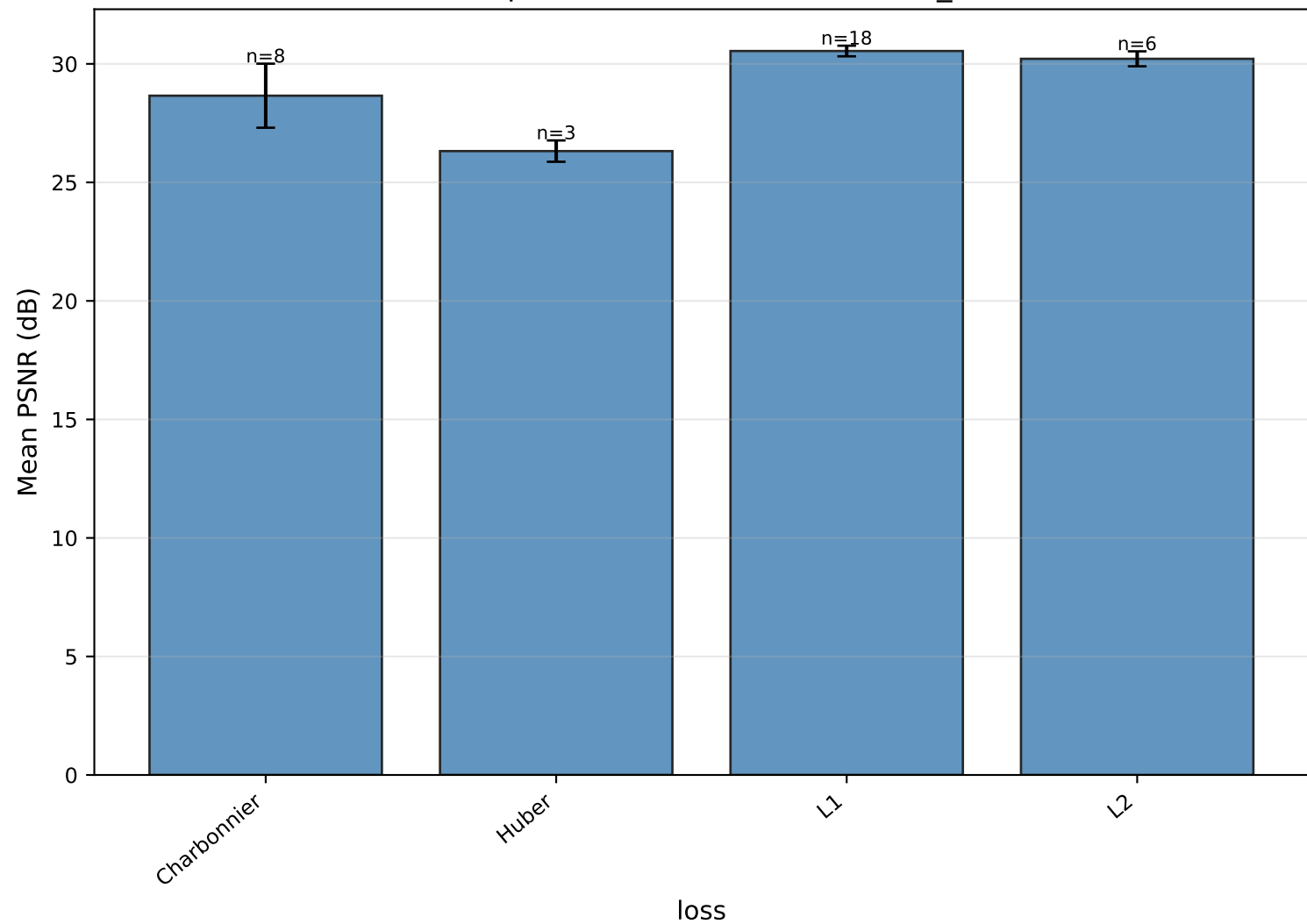
Mean PSNR per value of loss — DHTCUN_baseline
